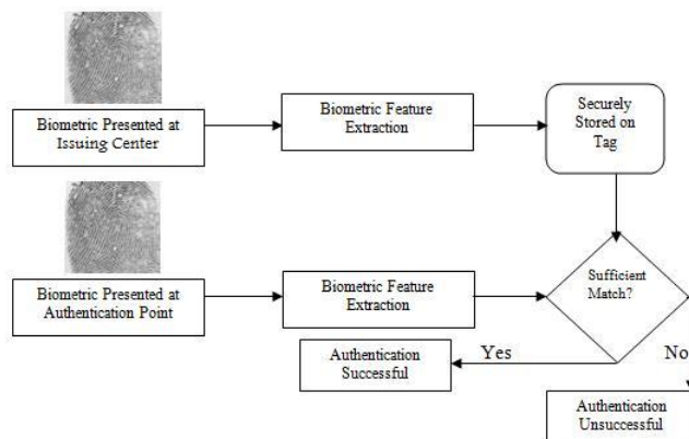
Fig. 1. Biometric Authentication
