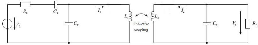
Fig. 2. HF RFID Equivalent Circuit
